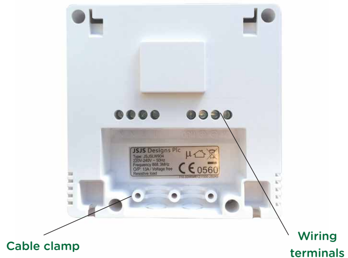
Typical wiring
