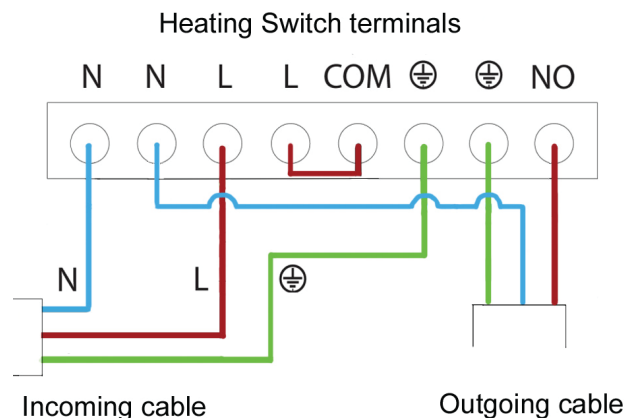
Typical wiring
