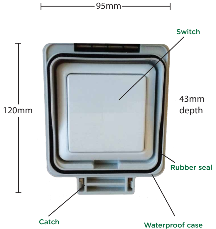
Cover open
